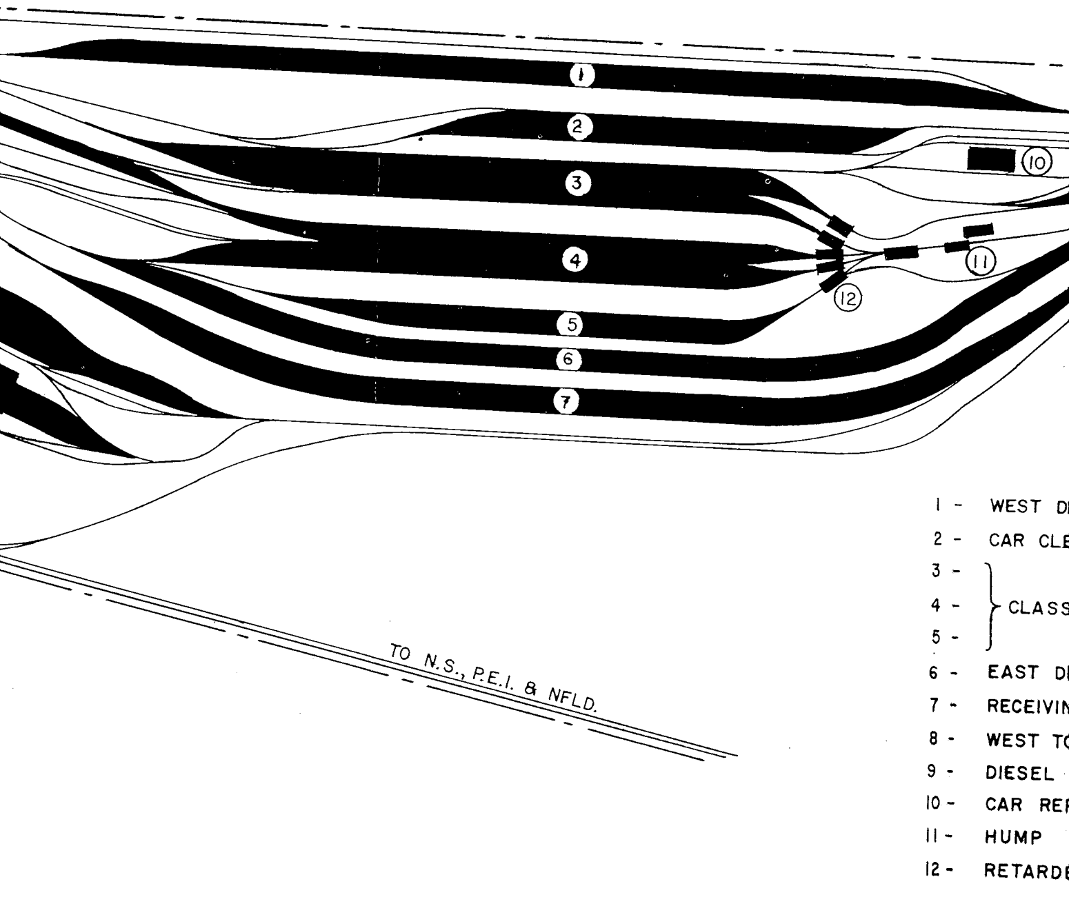
GENERAL PLAN OF C.N.R. MONCTON YARD
